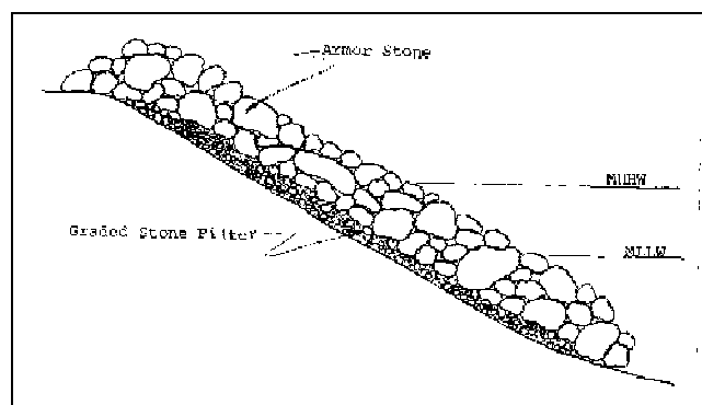
Figure B-2. Quarrystone revetment cross section
