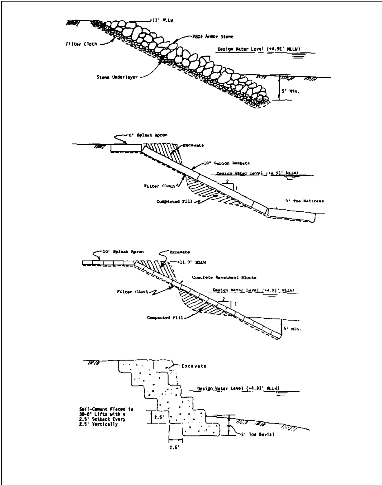
Figure E-2. Revetment section alternatives
