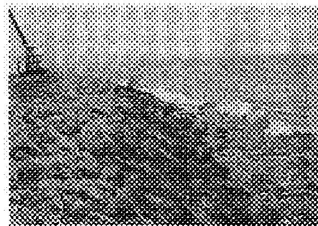
Figure B-1. Quarrystone revetment at Tawas Point, MI
